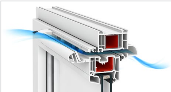
Aereco EMM humidity sensitive air inlet
