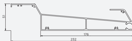
Lame orientable
